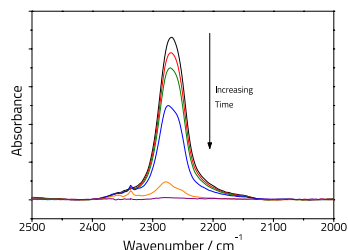
Decay in the N=C=O isocyanate band of a setting adhesive over time measured on an Arrow™ Si ATR slide
